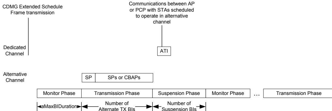
Figure 10-57a—Opportunistic transmission in alternative channels for CDMG STAs
