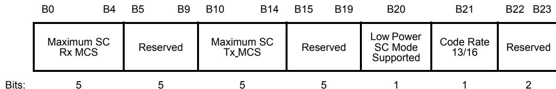
Figure 9-589cl—Supported MCS Set subfield format
