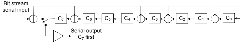
Figure 25-10—8-bit CRC calculation
