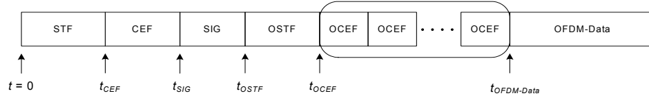
Figure 25-3—Packet structure for the OFDM mode PPDU
