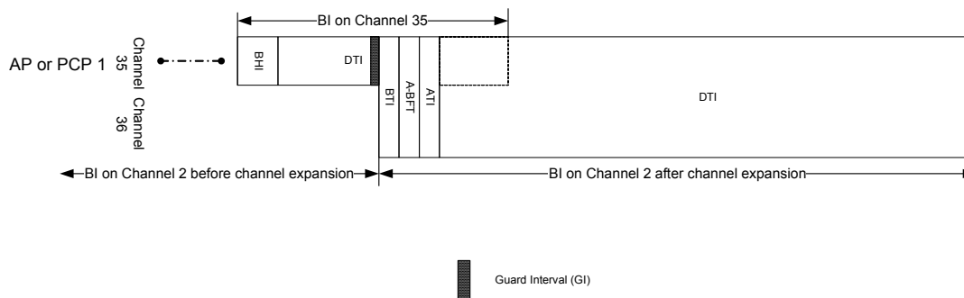
Figure 10-110—AP or PCP operating on channel 35 with independent beacon interval expanding the operating bandwidth to channel 2
