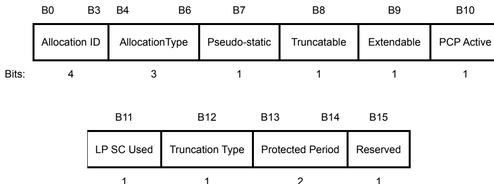
Figure 9-518a—Allocation Control subfield format (CDMG)
