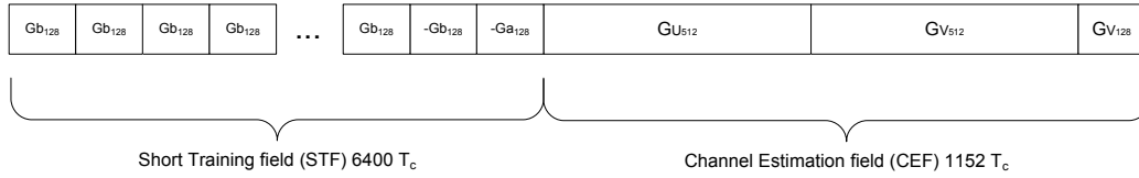
Figure 24-5—CDMG control mode preamble
