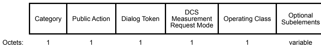
Figure 9-687f—DCS Measurement Request frame Action field format
