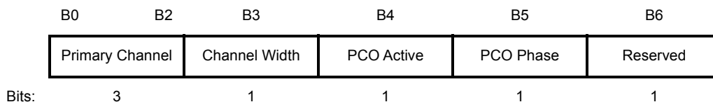
Figure 9-589do—CMMG Operation Information field
