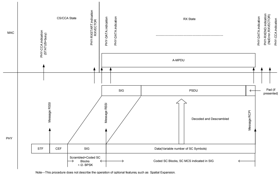
Figure 25-38—PHY receive procedure for a CMMG SC mode transmission
