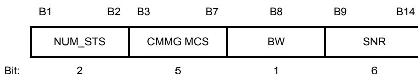
Figure 9-15c—MFB subfield in the CMMG Control field
