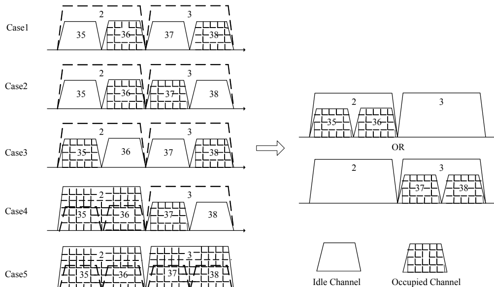
Figure 11-54—Examples of using DCS procedure
