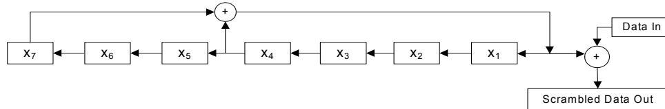
Figure 25-11—Scrambler
