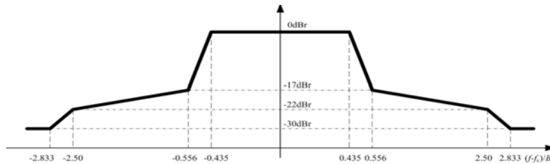
Figure 25-34—Example transmit spectral mask for a PPDU
