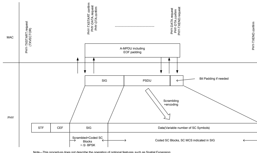
Figure 25-35—PHY transmit procedure for a CMMG SC mode transmission
