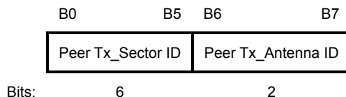
Figure 9-589db—Peer TX Antenna Parameter field format
