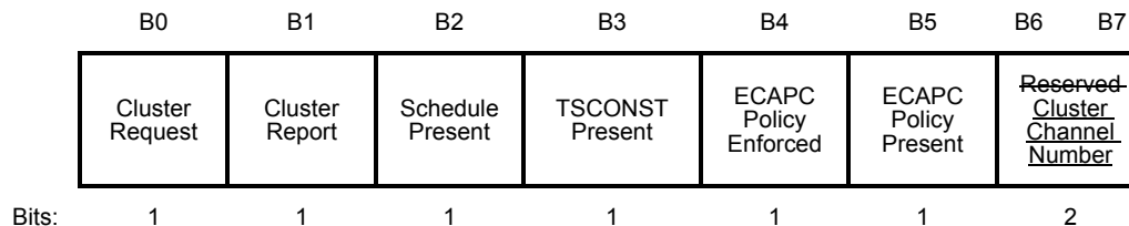
Figure 9-541—Cluster Report Control field format
