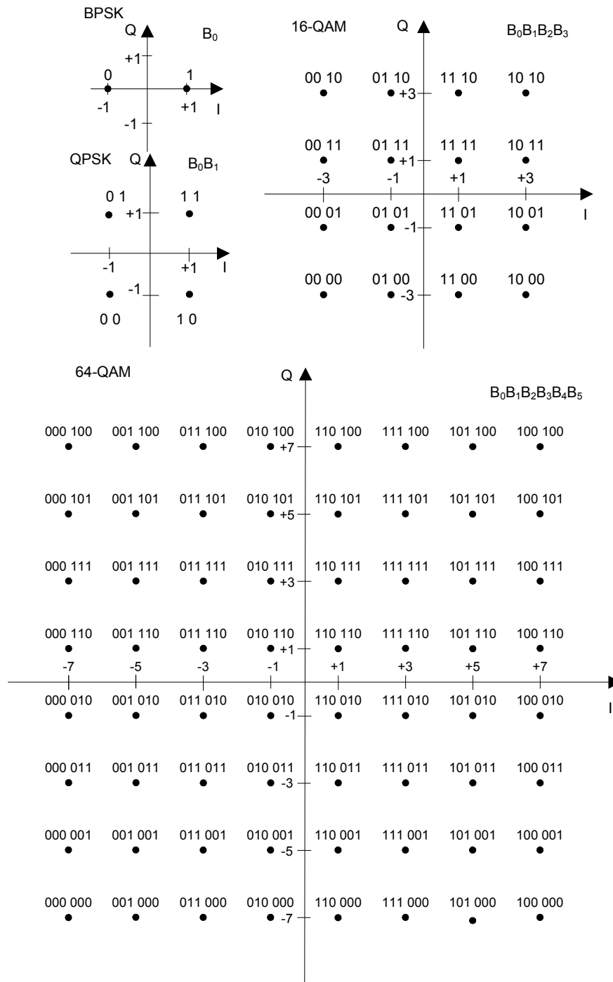
Figure 25-26—BPSK, QPSK, 16-QAM, and 64-QAM constellation bit encoding
