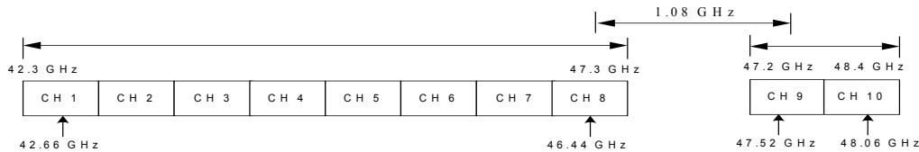
Figure 25-32—Channelization for CBW 540 MHz
