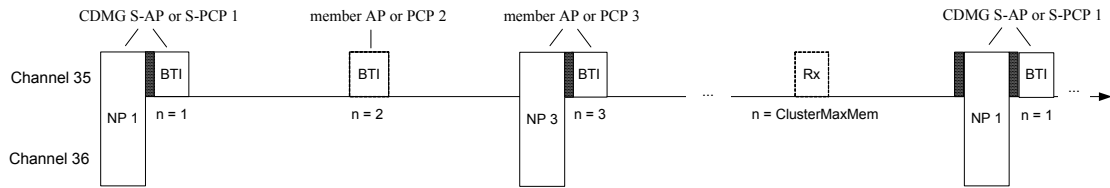
Figure 10-58a—Example of a decentralized AP or PCP cluster on a 1.08 GHz channel
