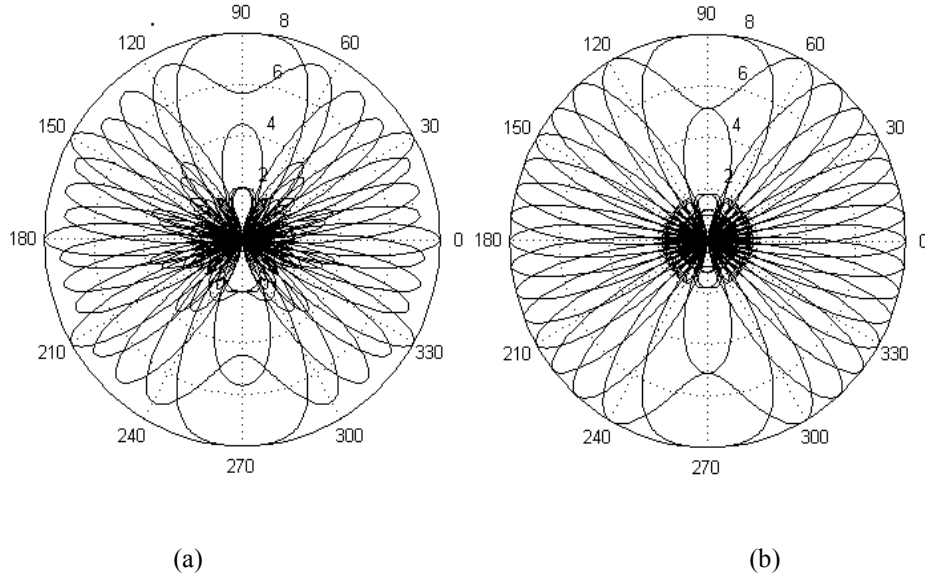
Figure W-2—Beam patterns generated by the codebook
