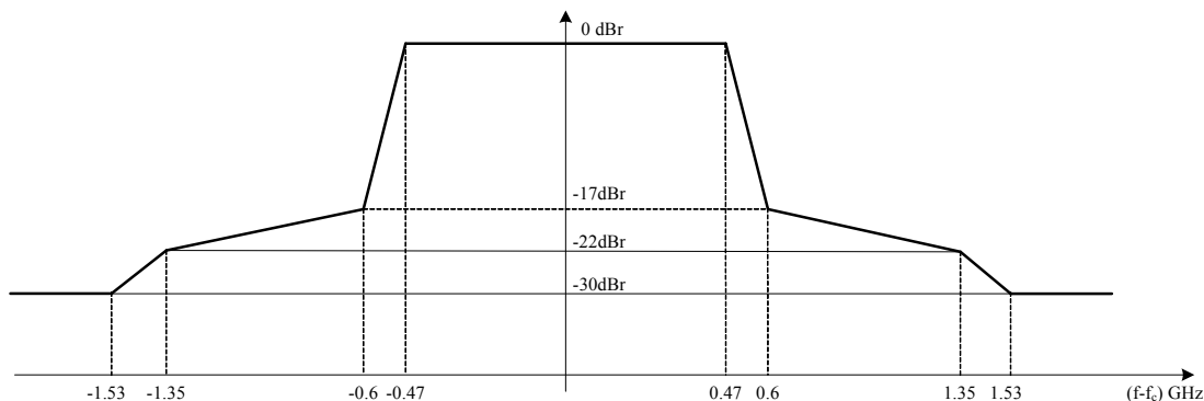
Figure 24-1—Transmit mask
