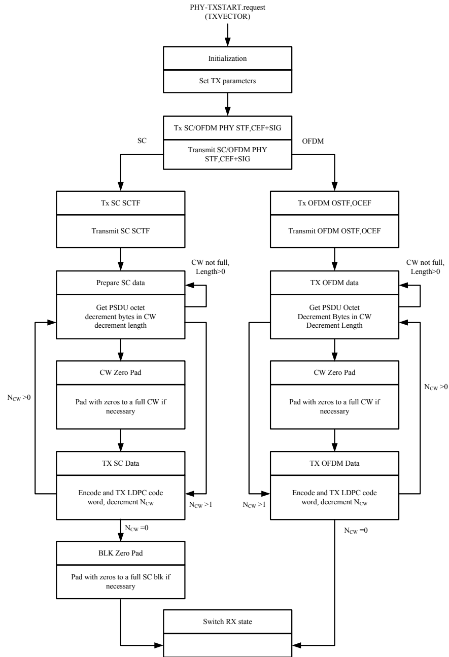
Figure 25-37—Typical Tx state machine
