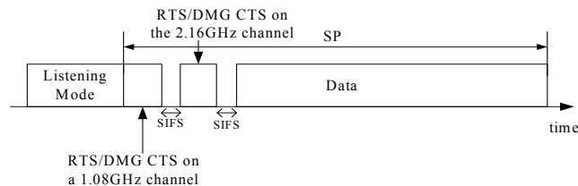
Figure 10-56a—An example of creating a CDMG protected period on two channels for CDMG STAs
