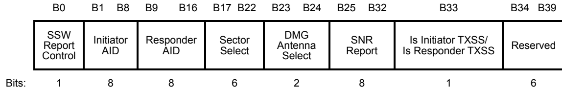
Figure 9-589cu—Report Info field format when the SSW Report Control subfield is 1
