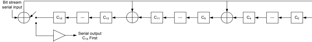
Figure 25-9—16-bit CRC calculation
