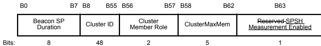
Figure 9-62—Clustering Control field format if the Discovery Mode field is 0
