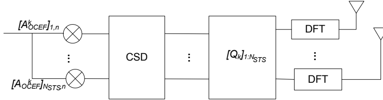
Figure 25-25—Generation of OCEF symbols per frequency segment
