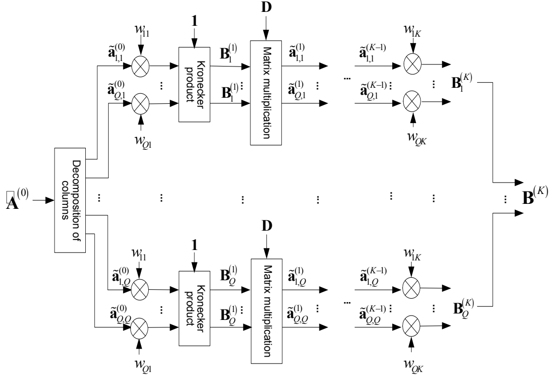
Figure 25-31—Generation of ZCZ sequences set
