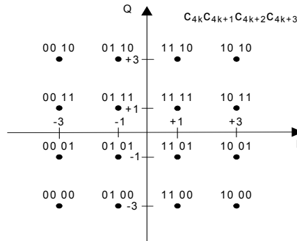
Figure 25-19—16-QAM constellation bit encoding
