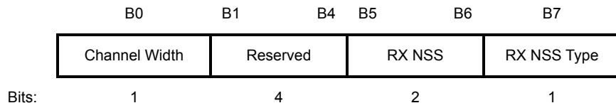
Figure 9-121e—CMMG Operating Mode field
