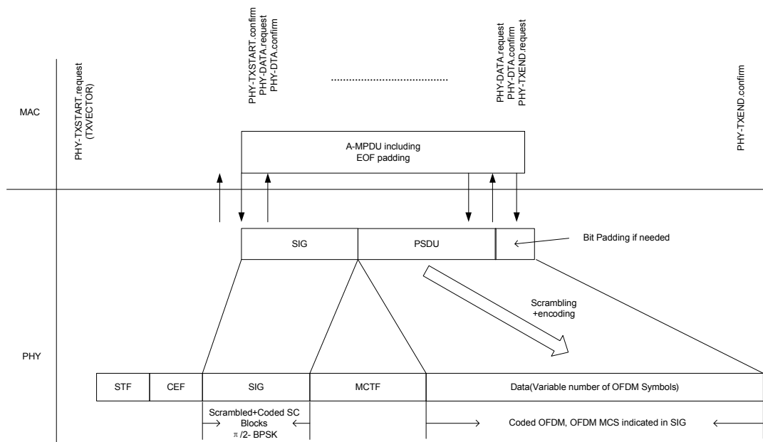
Figure 25-36—PHY transmit procedure for a CMMG OFDM mode transmission
