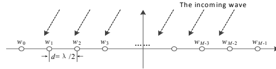
Figure W-1—An arrange mode of 1-D uniform linear antenna array
