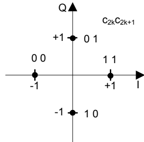
Figure 25-18—QPSK constellation bit encoding
