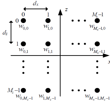
Figure W-3—An arrange mode of 2-D uniform linear antenna array
