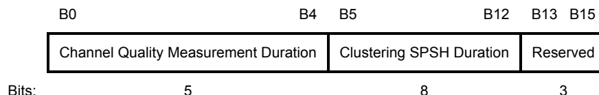
Figure 9-589df—Clustering SPSH Control field format
