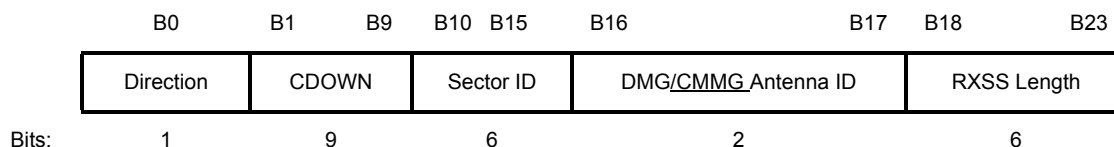
Figure 9-635—SSW field format
