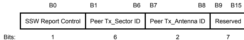
Figure 9-589cv—Report Info field format when the SSW Report Control subfield is 0
