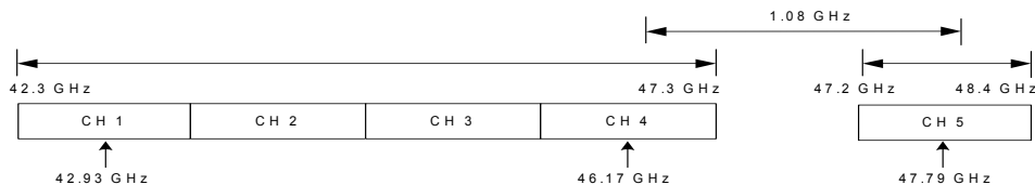
Figure 25-33—Channelization for CBW 1080 MHz
