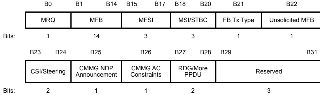
Figure 9-15b—CMMG Control field
