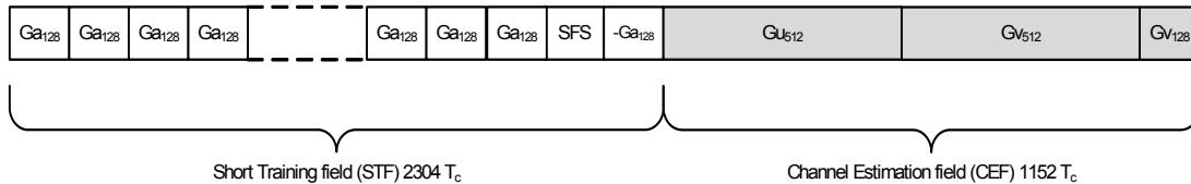
Figure 24-2—CDMG SC mode preamble
