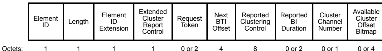
Figure 9-589cx—Extended Cluster Report element format
